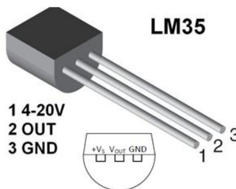
Figure 4: LM35 Sensor
